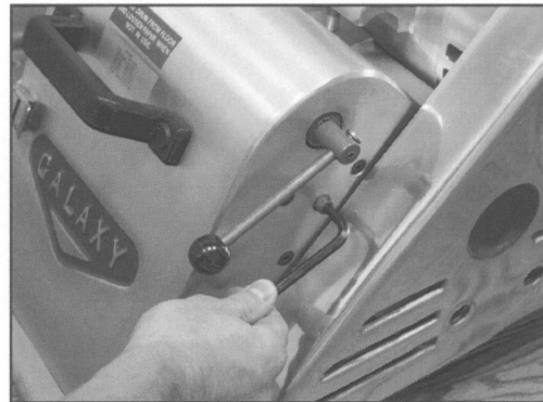
26. Turn adjustment screw as required.
