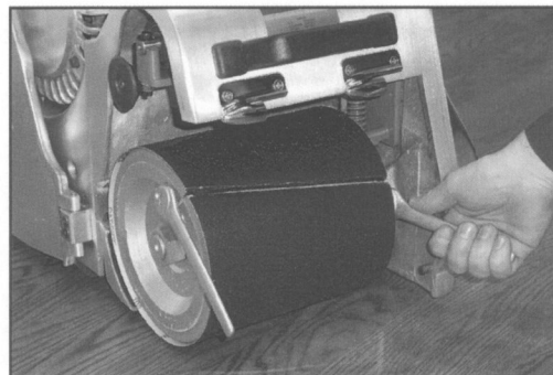
19. Tighten firmly.
